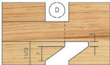
Chanfrein 36°
