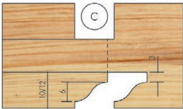
Talon 10x6
